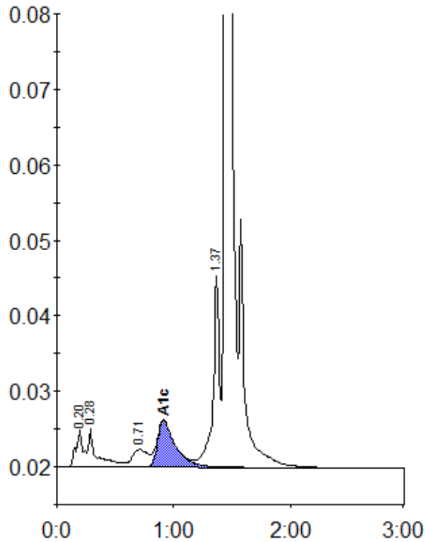
Peak table - ID: 10461018
